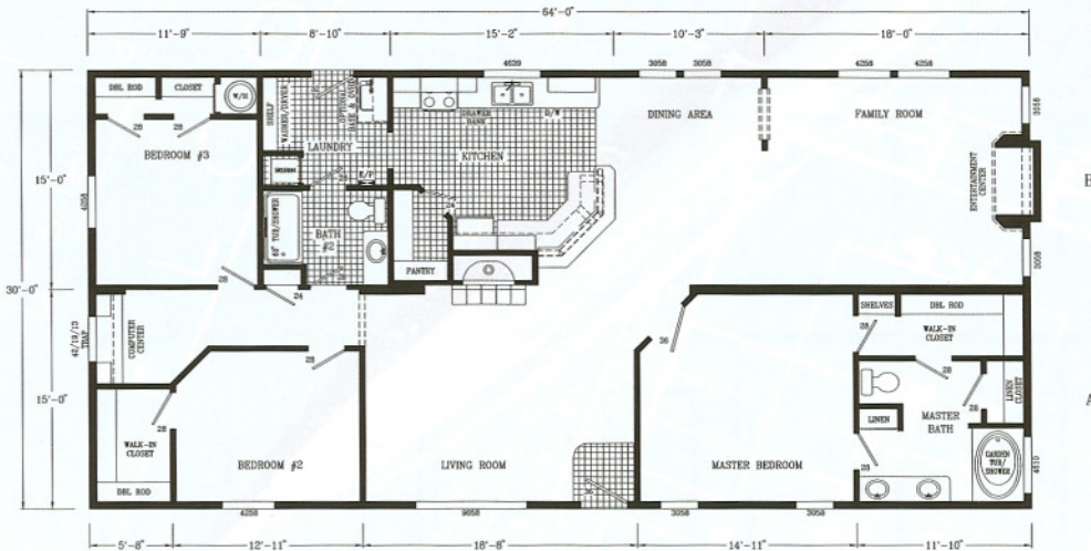
PLAN 545 6832 3FMBB APPROX. 1,920 SQ. FT.
